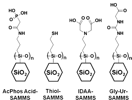
FIGURE 1. Schematic of the organic ligand monolayers utilized in this study.
